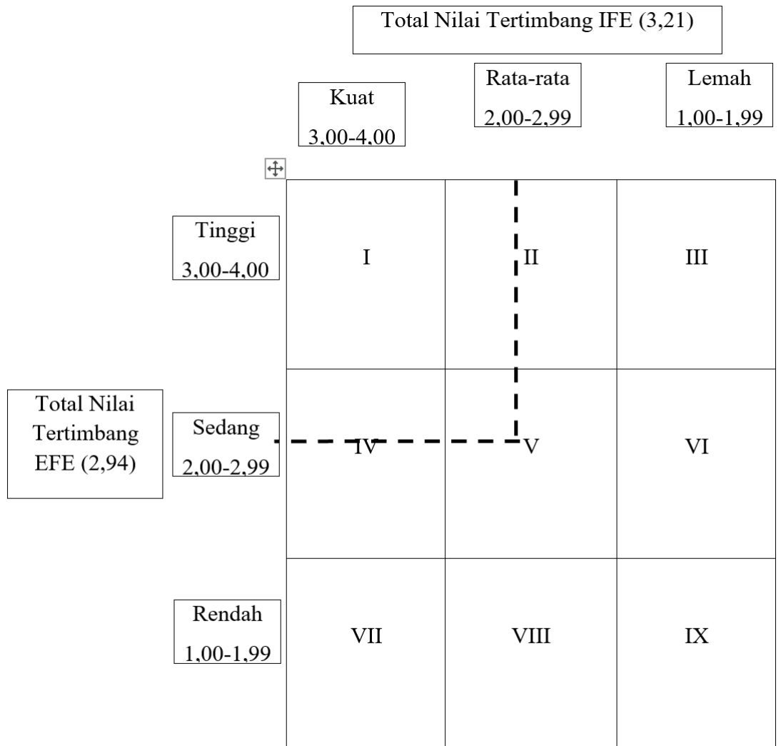
Gambar 4. 3 IE Matriks
