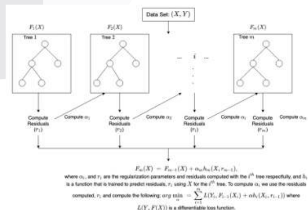
GAMBAR 3 cara kerja XGBoost (sagemaker XGBoost docummentation)
