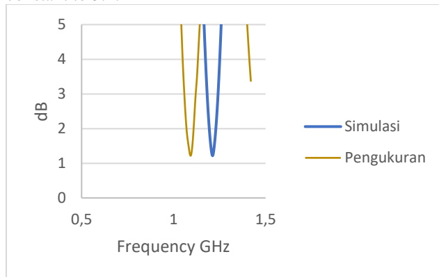
FIGURE 17 VSWR on ADS-B antenna
