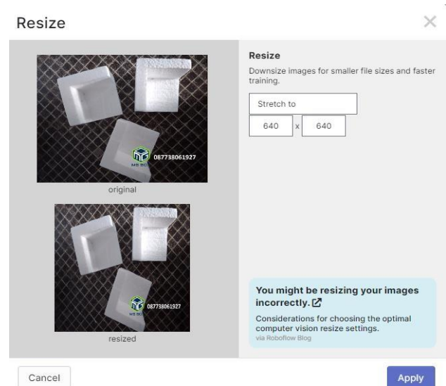
GAMBAR IV.4. Pre-Processing Dataset
