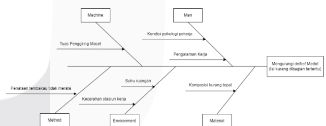
GAMBAR 2 Fishbone Diagram
