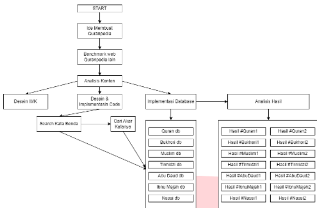
GAMBAR 1 Flowchart Quranpedia
