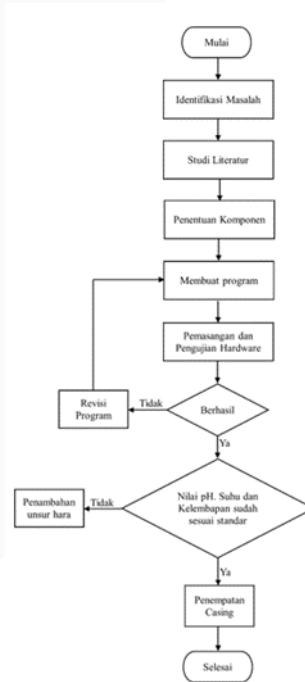
GAMBAR 3.2 Flowchart Sistem
