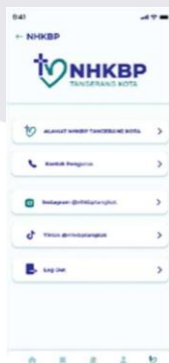
Gambar 4.31 Tampilan NHKBP
