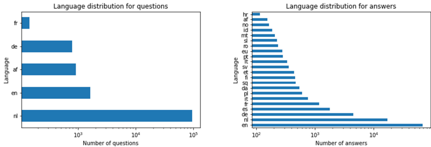
Fig. 1. Language distribution for questions and answers of the Dutch SQuAD v2.0 dataset. All languages are shown that exceed the threshold value t = 100 .
