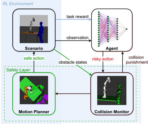
Fig. 1. Our MoveRL framework. Our safety layer leveraging the MoveIt motion planner contains 2 modules: 1) a collision monitor, that detects actions that lead to collisions, and 2) a motion planner, that plans a collision-free path to reach the target locations encoded in (previously-identified) safe actions.
