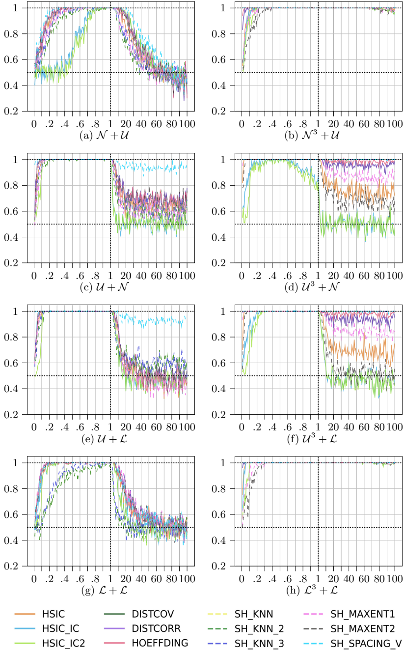
Fig. 1. Several selected detailed results for Resit. x -axis shows the values of i -factor and y -axis shows the accuracy of causal identification.
