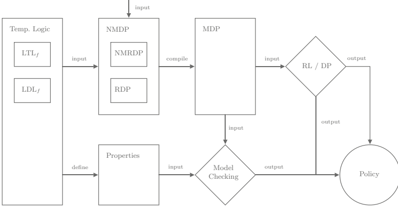
Fig. 2. Conceptual/tool chains
