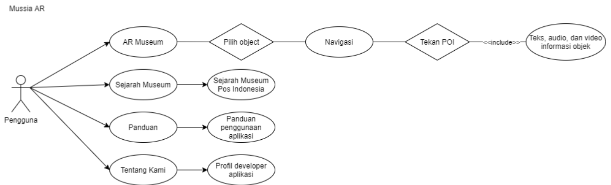
Gambar 3. 2 Use Case Diagram
