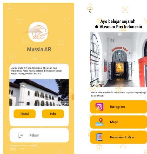
Gambar 4. 6 Pop-Up Jarak
