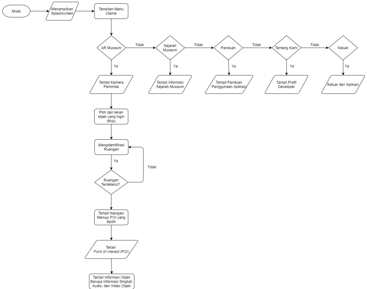
Gambar 3. 3 Flowchart
