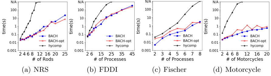
Fig. 11. Experimental results in reachable models
