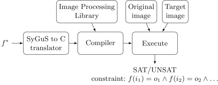
Fig. 5. Oracle for image transformations
