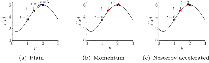
Fig. 4. Different GD methods on f for R = [0, 3]
