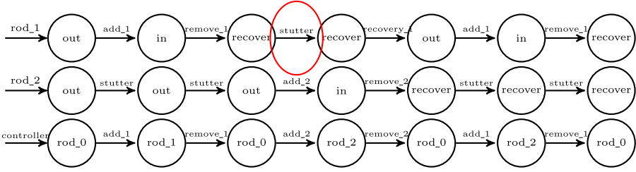
Fig. 9. Path of randomly waiting
