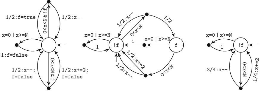
Fig. 4. Left: The coin game as a single-location PCFP \mathfrak{P}_{\text{game}} . Middle: The PCFP after unfolding variable f . Right: The PCFP after eliminating the location labeled f .
