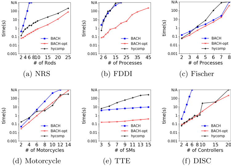
Fig. 12. Experimental results in unreachable models
