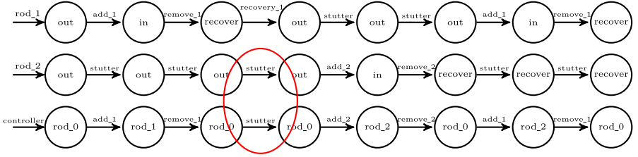
Fig. 8. Path of repeated waiting for shared labels
