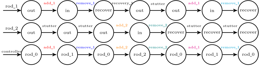
Fig. 3. Path \rho_{step} in the step semantics of CLHA from Fig. 2
