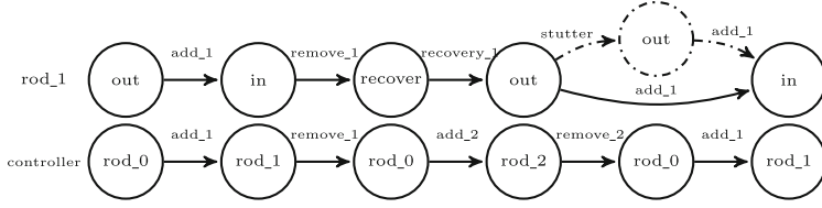
Fig. 6. Infeasible path segment in \rho_{\text{shallow}} and \rho_{\text{step}}
