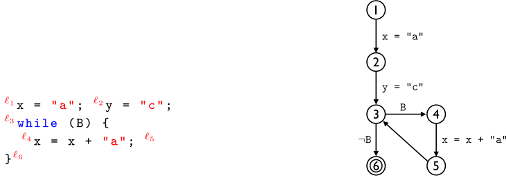
Fig. 3. Example of CFG generation.
