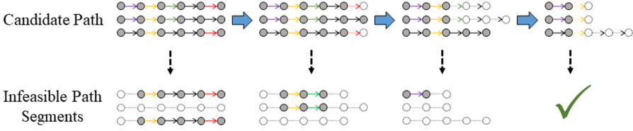
Fig. 10. Path splitting to obtain multiple infeasible path segments
