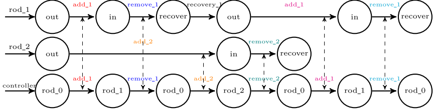
Fig. 5. Candidate path \rho_{shallow} in the shallow semantics
