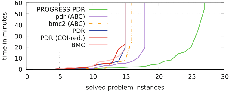
Fig. 4. Results on deep counterexamples.
