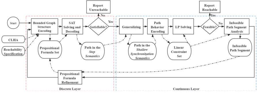
Fig. 1. Mixed semantics guided layered bounded reachability analysis
