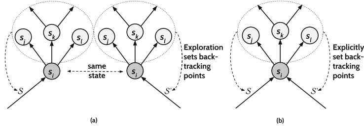
Fig. 2. (a) Stateless model checking explores s_i , s_j , s_k , and s_l twice and thus sets backtracking points for both \mathcal{S} and \mathcal{S}' . (b) Stateful model checking matches state s_i and skips the second exploration and thus we must explicitly set backtracking points.
