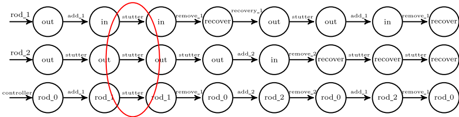
Fig. 7. Path of global waiting
