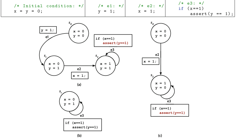
Fig. 5. Example of an event-driven program for which a naive application of the standard DPOR algorithm fails to construct the correct persistent set at state s_0 . We assume that e_1 , e_2 , and e_3 are all initially enabled.
