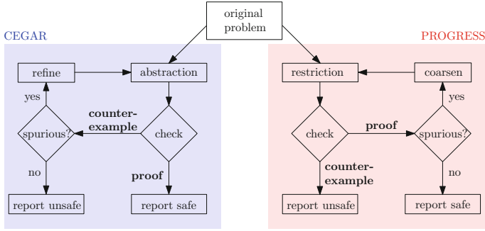
Fig. 1. Comparing CEGAR and PROGRESS.
