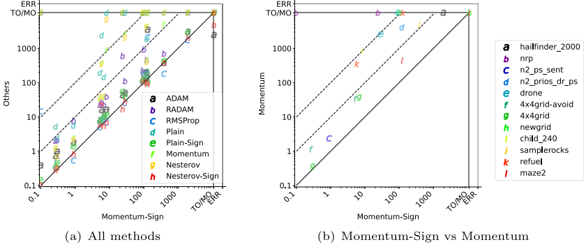
Fig. 6. Comparison of different GD methods
