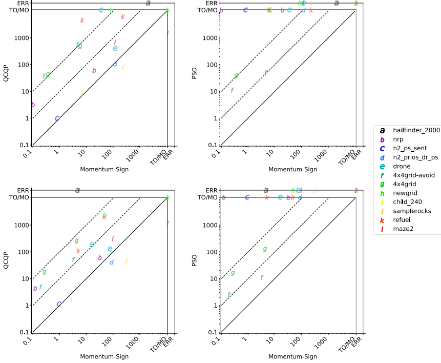
Fig. 7. Comparison of GD with QCQP and PSO against optimum-bounds (upper) and 20% relaxed-bounds (lower)
