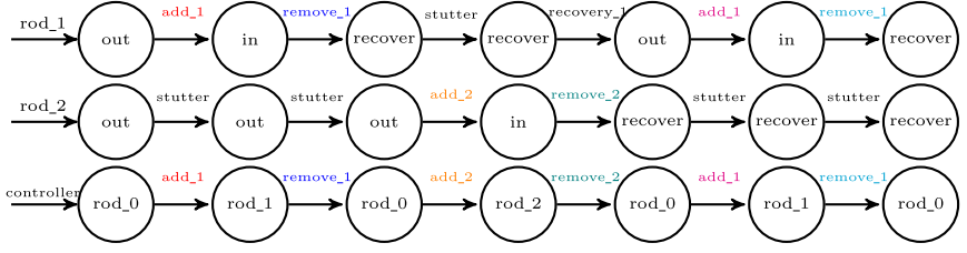
Fig. 4. Path \rho'_{step} obtained by changing the order of recover_1 and stutter in \rho_{step}
