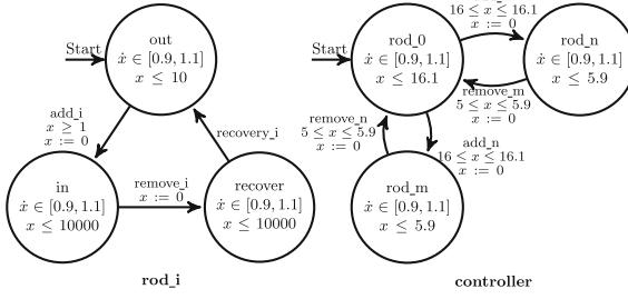
Fig. 2. Nuclear reactor system
