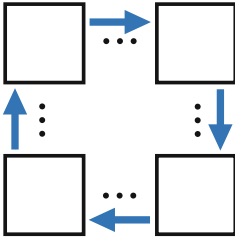
Fig. 5. Abstract moves
