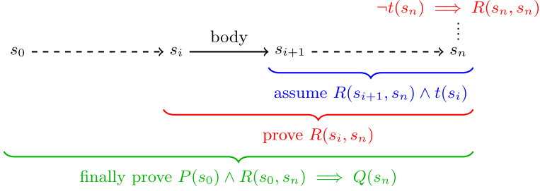
Fig. 3. Backward propagation conditions for a loop postcondition R with respect to an iteration of the loop. The overall conclusion is marked green. (Color figure online)
