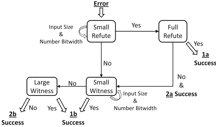
Fig. 2. BSQCHK checker workflow.
