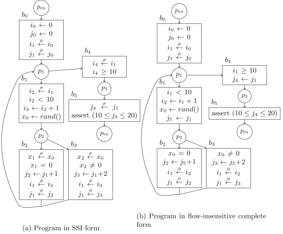
Fig. 3. Comparison of the SSI form and the FIC form of the program from Fig. 2
