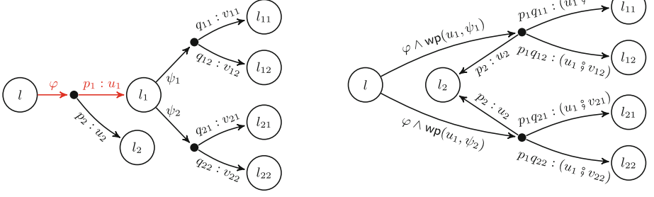
Fig. 6. Transition elimination in PCFPs. Transition l \xrightarrow{\varphi \rightarrow p_1:u_1} l_1 is eliminated. The rule is correct even if the depicted locations are not pairwise distinct.
