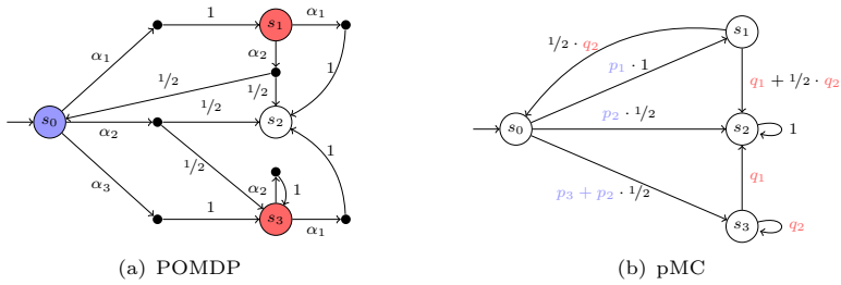
Fig. 2. From POMDPs to pMCs [32, p. 182].
