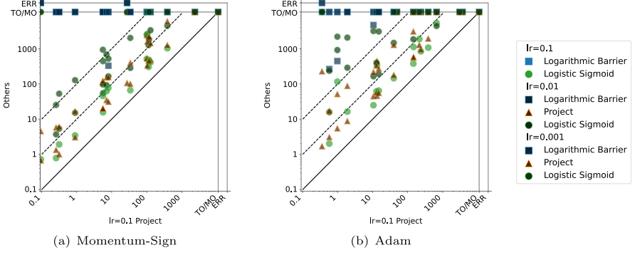
Fig. 5. Comparison of different region restriction methods
