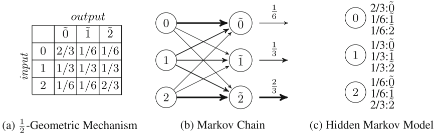
Fig. 1. Truncated \frac{1}{2} -geometric mechanism
