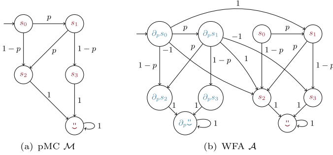
Fig. 3. A (left) sample parametric MC and (right) its derived weighted automaton
