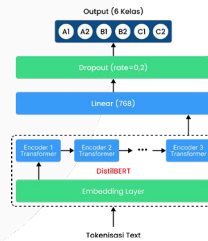
Gambar 7. Arsitektur DistilBERT matriks Lexical
