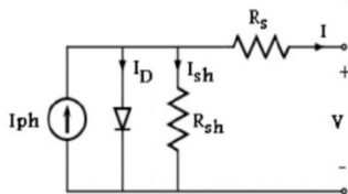
GAMBAR 2.4 equivalen circuit diagram [5]
