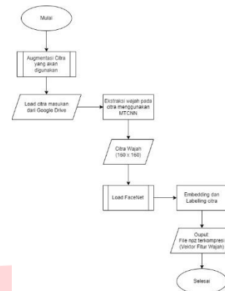
GAMBAR 1 (Flowchart praproses)
