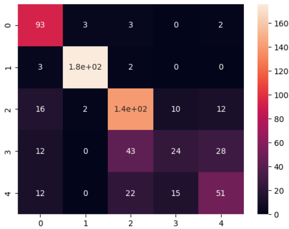
GAMBAR 4.4: Confusion Matrix
