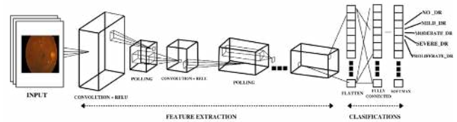
GAMBAR 3.1: perancangan sistem machine learning
