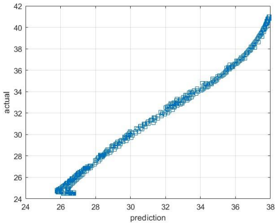
Figure 2. (a) the results of prediction data using the JST method on humidity data
