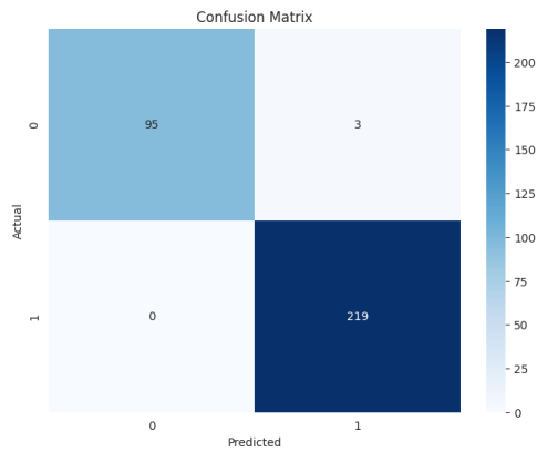
Gambar 2. Confusion Matrix
