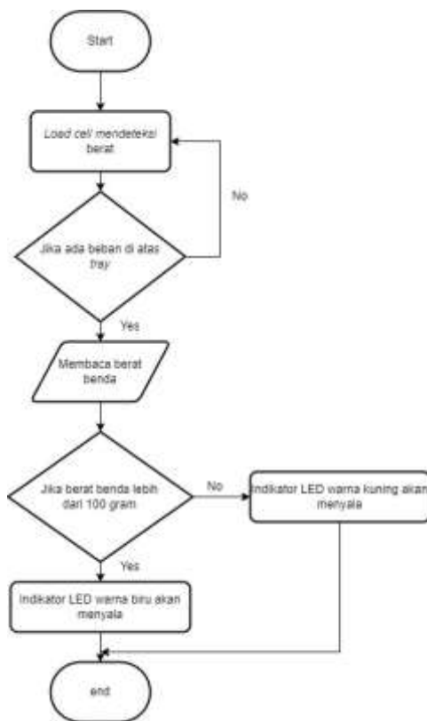
Gambar 3. 4 Flowchart sistem
