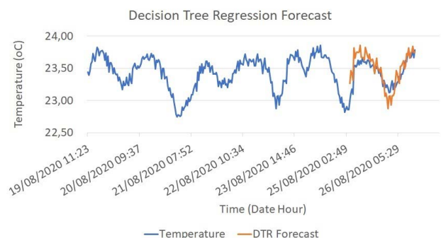
FIGURE 4. DTR forecast.
