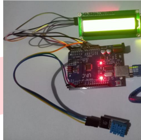
GAMBAR 1. Setup Penelitian
