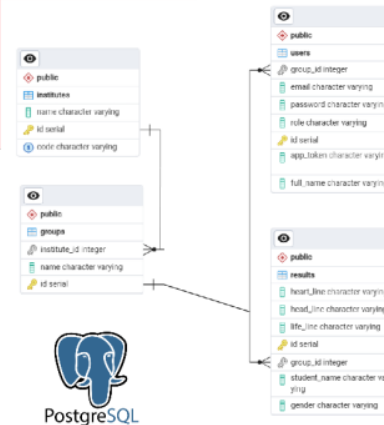
Gambar 2. Database Entity Relationship Diagram.
