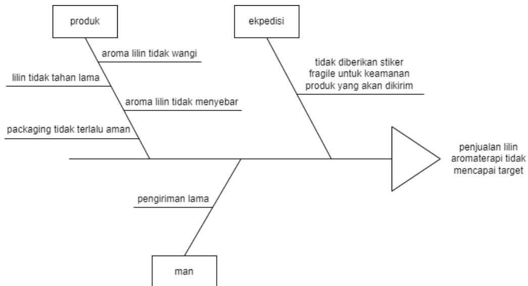
Gambar I. 3 Diagram fishbone
