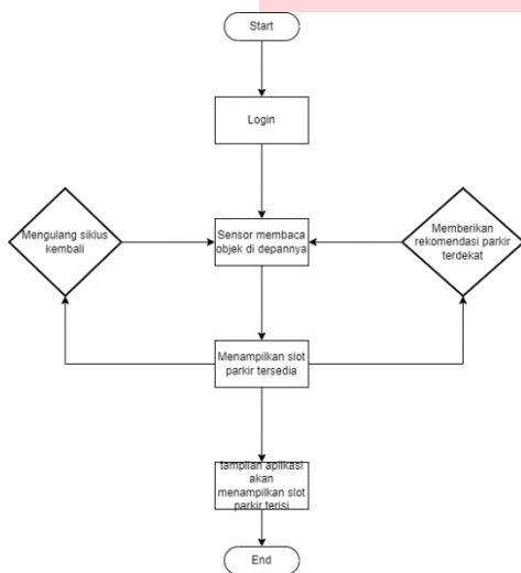
Gambar 3. 1 Flowchart
