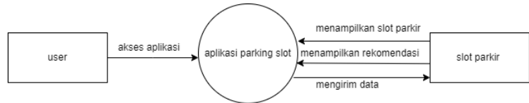
Gambar 3. 3 DFD level 0
