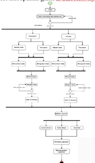
GAMBAR 4 Activity Diagram
