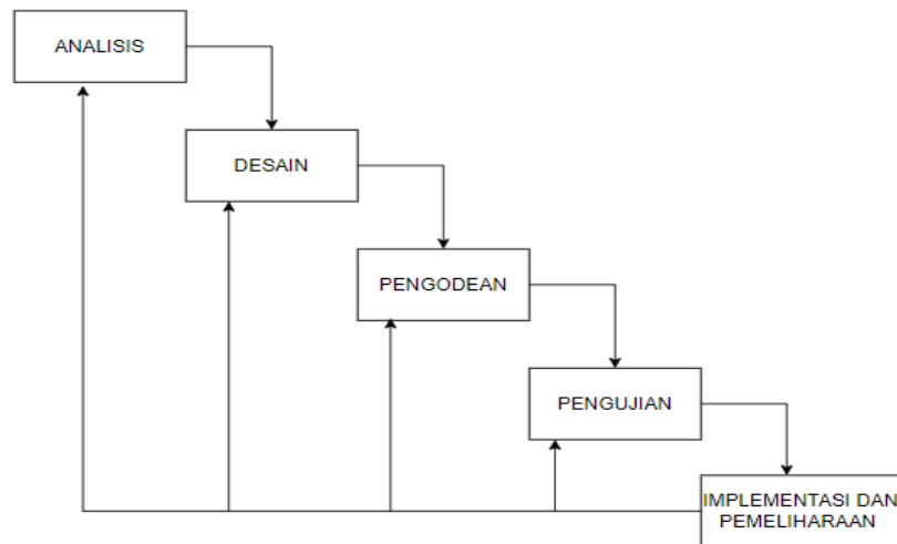
Gambar 1. 1 Metode Waterfall
