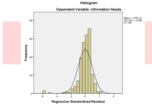
Figure 2. Normality Test Results Normal Probability Histogram Source Processed SPSS Data (2024)
