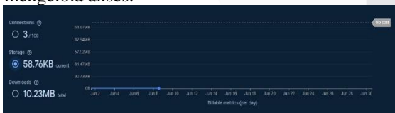
GAMBAR 1.4 Storage Firebase
