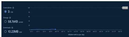
GAMBAR 1.3 Connections Firebase
