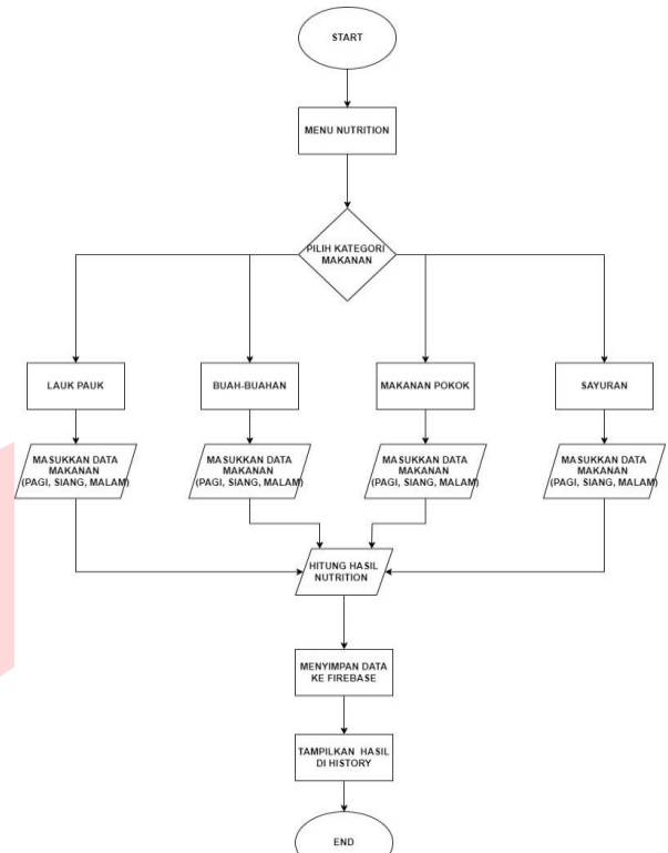
GAMBAR 6 Flowchart menu nutrition .
