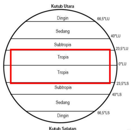
Figure 1.1 Solar Climate [2]
