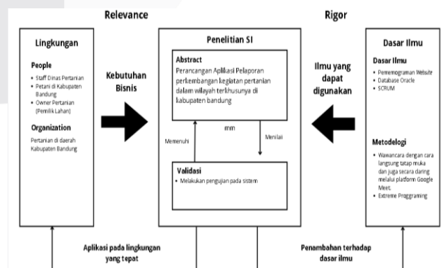
Gambar 2 : Model Konseptual
