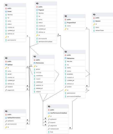
GAMBAR 6 Entity Relational Diagram
