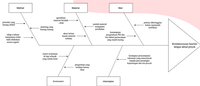
GAMBAR 3 Diagram Fishbone
