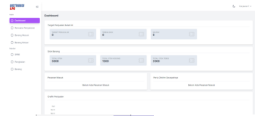
Gambar 11 (Halaman Dashboard)
