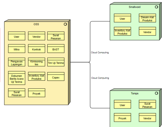
Gambar 6 Data Dissemination Diagram
