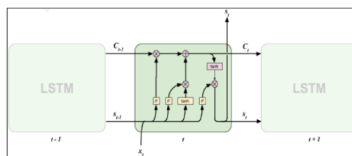
Gambar 1. Memory Cell LSTM [8]
