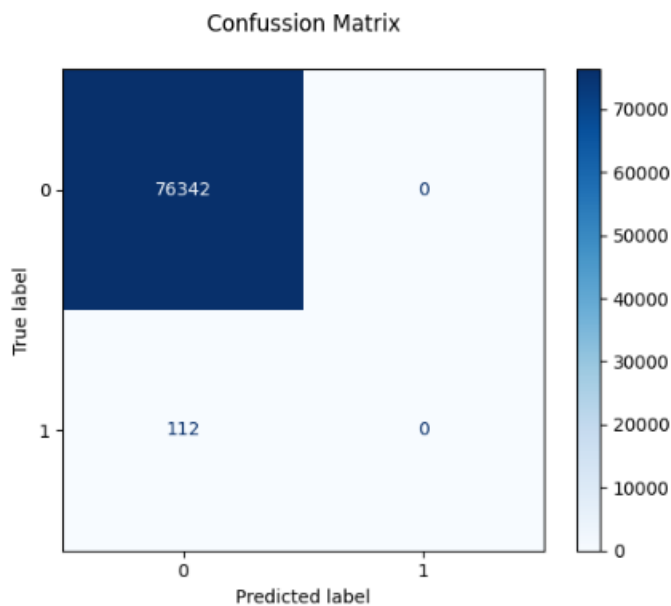
Gambar 10. Confusion Matrix Bi-LSTM
