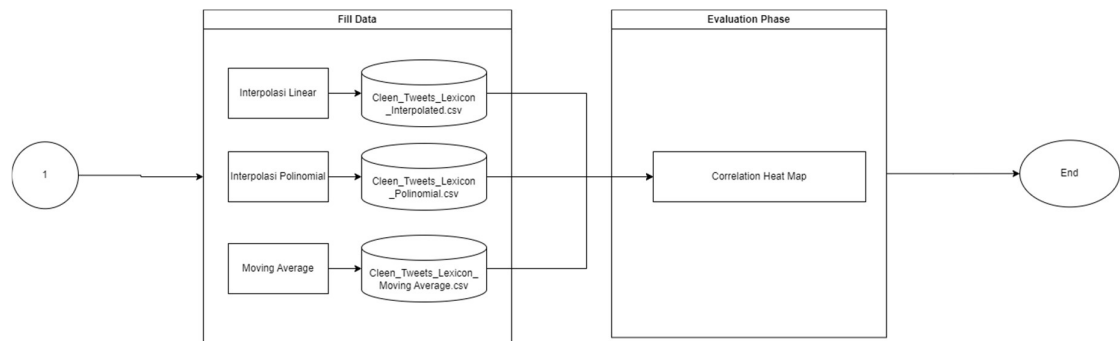
Gambar 3.2 Flowchart
