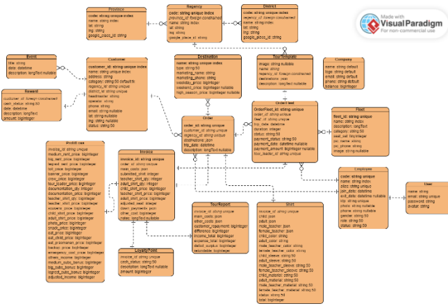
GAMBAR 3 Entity Relationship Diagram Aplikasi Divisi Marketing
