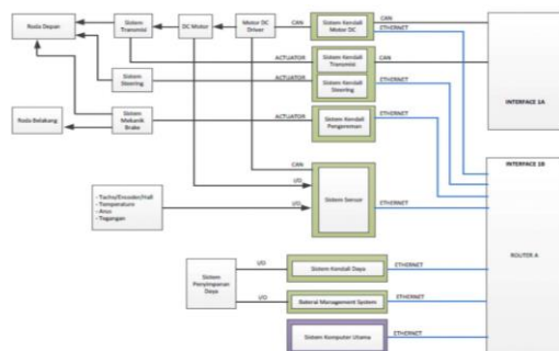
Figure 2.1 Electric Vehicle Block Diagram for CAN
