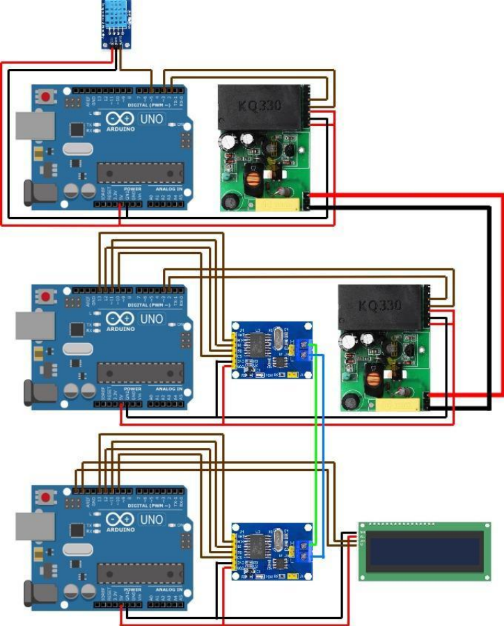
Figure 4. Wiring Diagram of Full System of EVPLC Module Testing
