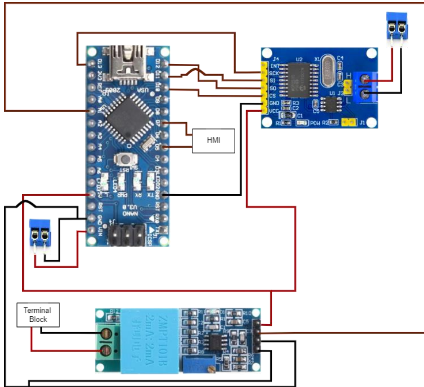
Figure 8. Wiring Diagram for EVCS Simulation PCB
