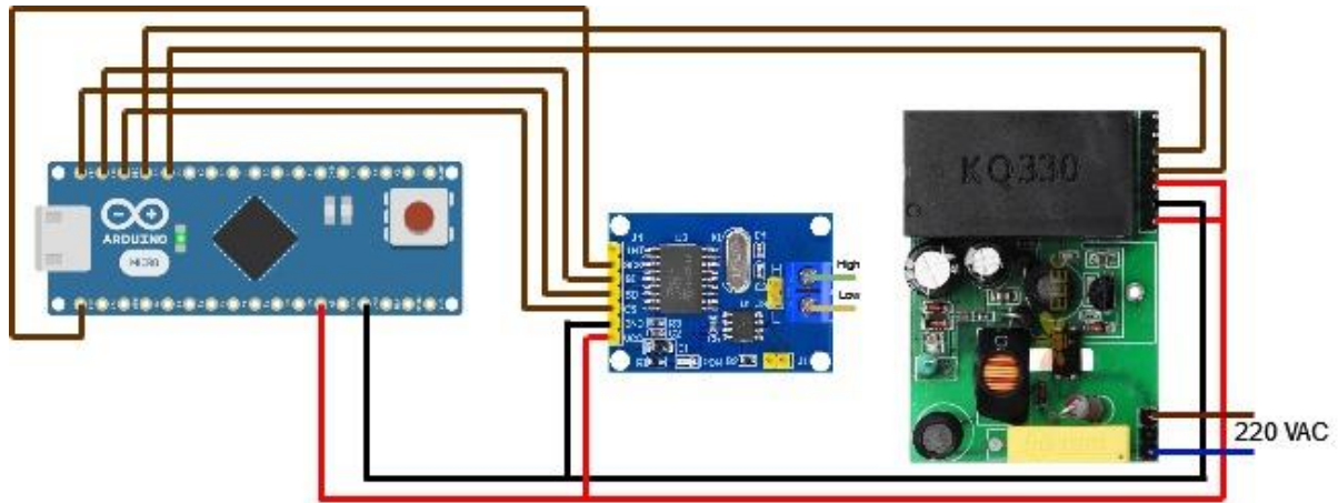
Figure 6. Wiring Diagram of EVPLC Module
