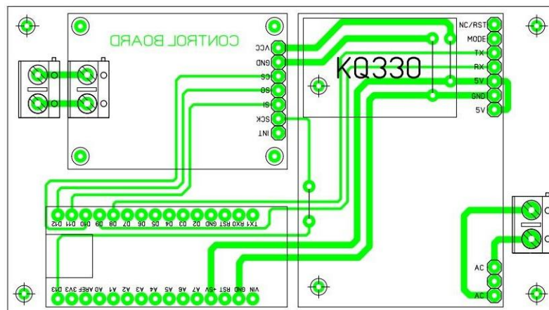
Figure 7. PCB Design for EVPLC Module
