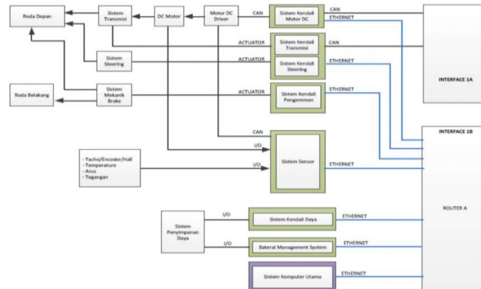
Figure 1. Electrical Vehicle Network Block Diagram for CAN
