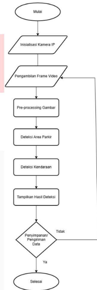
Gambar 7. Flowchart sistem
