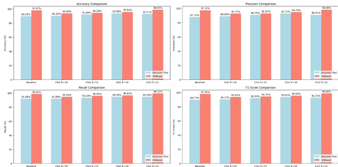
Gambar 4. Perbandingan Performa Metode Decision Tree dan XGBoost
