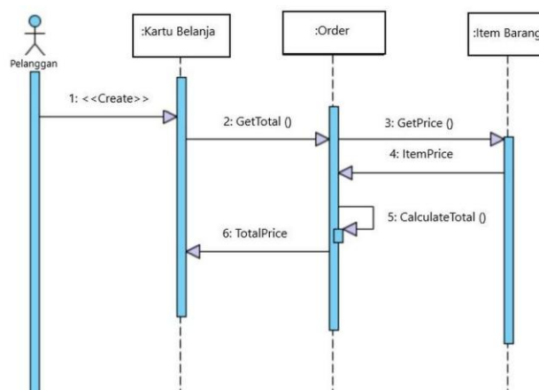
Gambar 2. 3 Sequence Diagram
