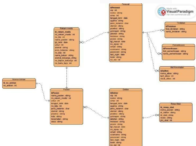
Gambar 16. Logical Data Diagram teraMedik
