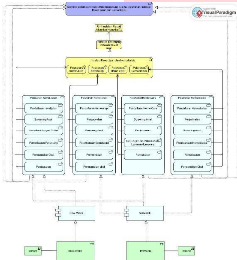
Gambar 3. Goal Diagram
