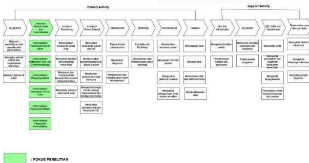
Gambar 5. Decomposition Diagram
