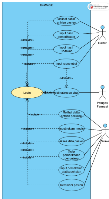
Gambar 20 Use Case Diagram teraMedik
