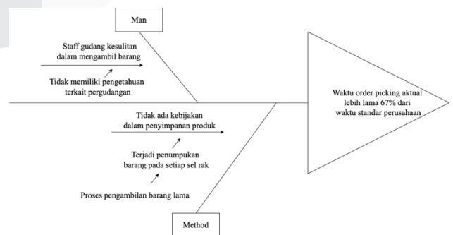
Gambar I. 5 Fishbone Diagram
