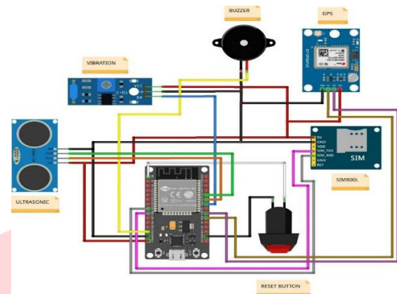
GAMBAR 5 Perancangan Hardware
