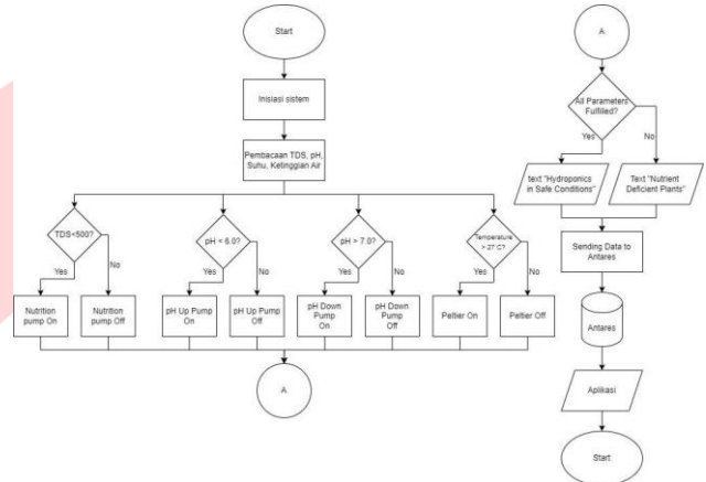
GAMBAR 6 Flowchart AWNDES
