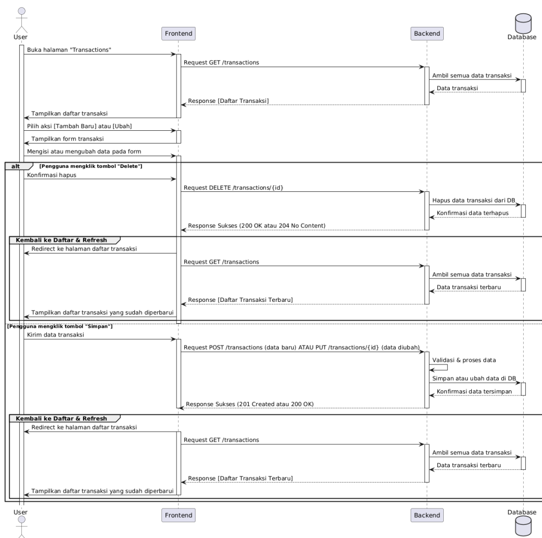
Gambar 4.16 Sequence Diagram Trasaction
