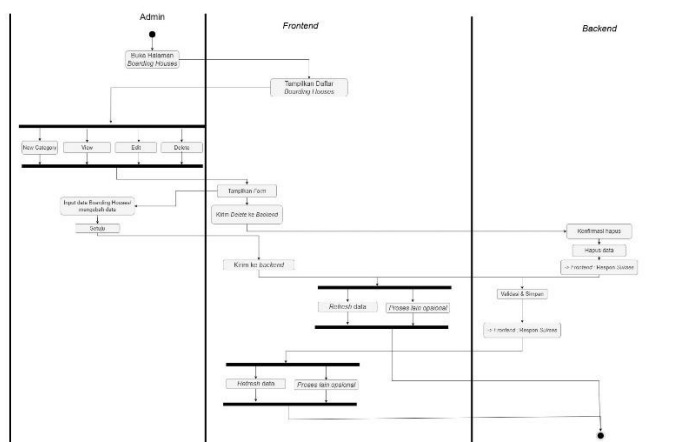
Gambar 4.5 Diagram Activity Menu Input Data Boarding Houses
