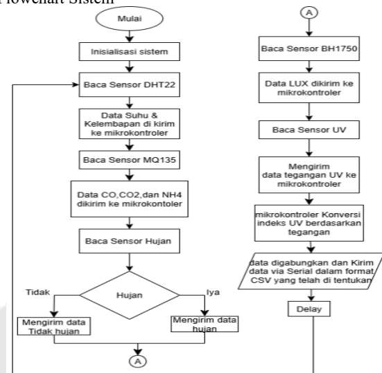
GAMBAR 2 Flowchart Sistem
