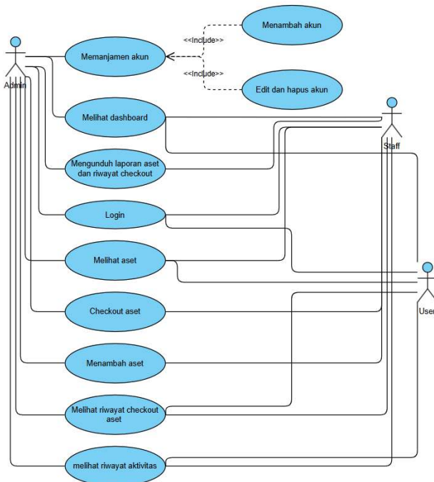
GAMBAR 2 Usecase Diagram
