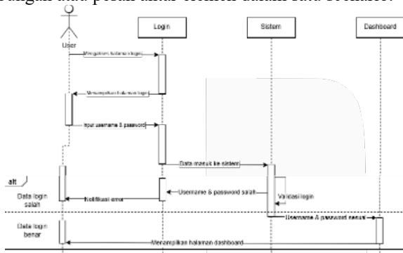
GAMBAR 5 Sequence Diagram
